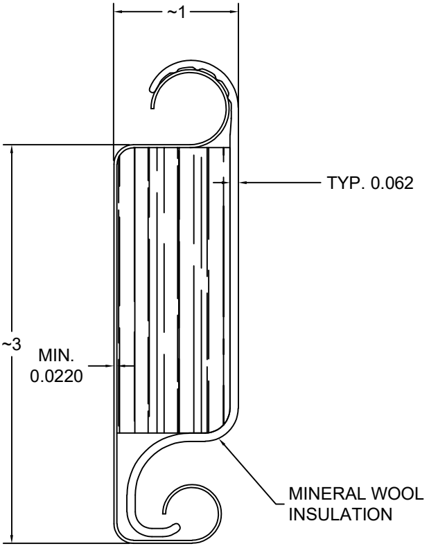
② SLAT DETAIL TYPICAL SECTION FRONT SLAT:
